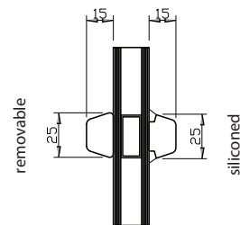
Vienna glazing bar with ghost bar: 25 mm
